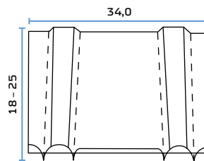
Wellennagel Typ W-Maxi Corrugated Fastener Type W-Maxi
