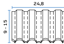
Wellennagel Typ W Corrugated Fastener Type W
